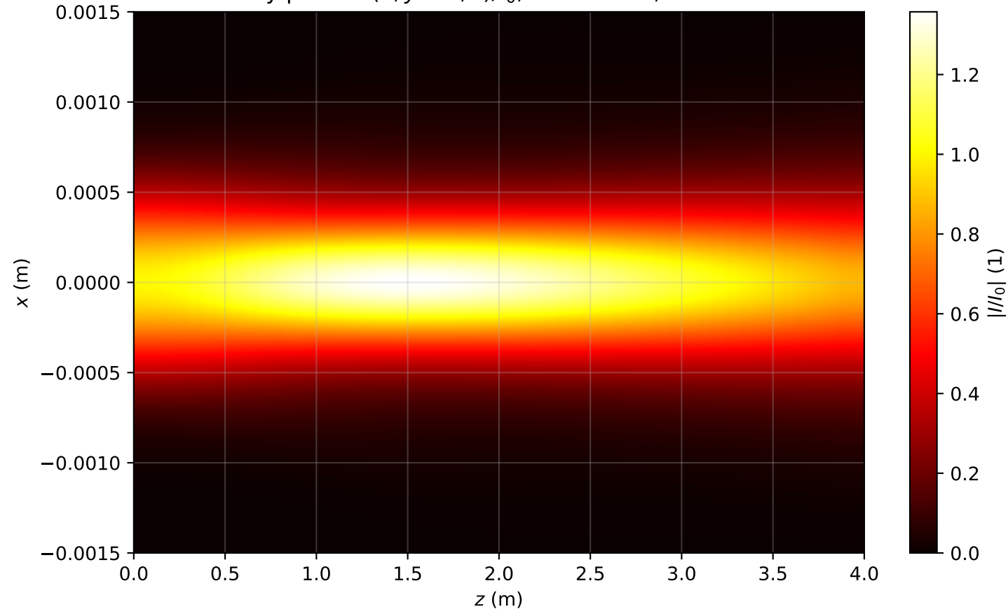
Intensity profile I(x, y = 0, z)/I_0 , P_{in}=0.8P_{cr} , artificial time
